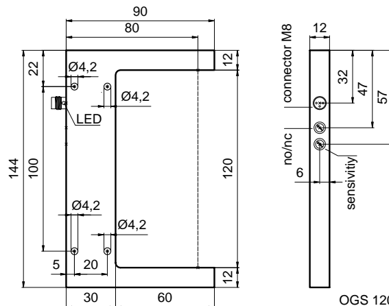
OGS 120 dimensions: mm
