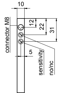
OGS 080 dimensions: mm
